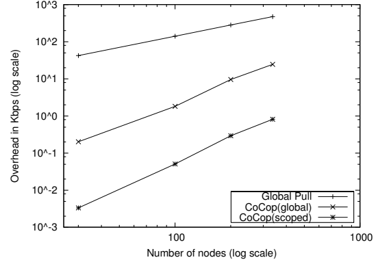
Figure 8: Variation of communication overhead with number on nodes
