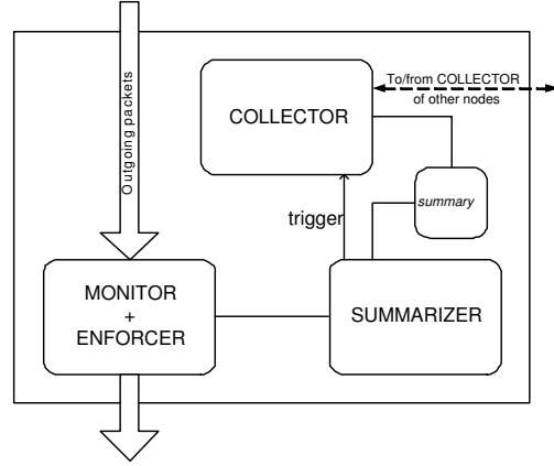
Figure 1: Components of pull-based CoCop at each node
