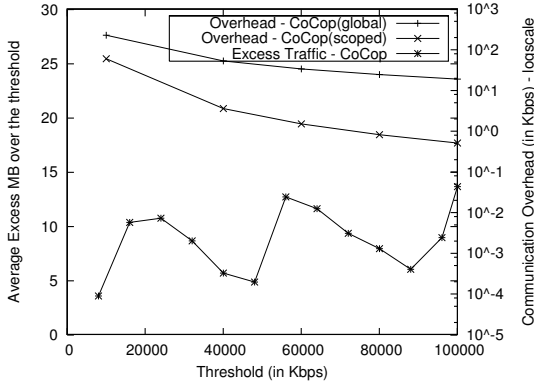
Figure 9: Effect of varying the threshold. Average Excess Bytes in the left y-axis and communication overhead on the right y-axis. While excess traffic shows no discernable trend, communication overhead increases as threshold decreases.
