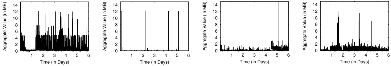
Figure 4: These figures show the temporal variation of four of the 42 aggregate flows that were anomalous at some point during the trace. In general, no common temporal characteristic is observed amongst the anomalous flows.
