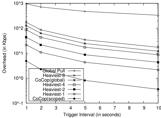
Figure 5: Communication Overhead. The overhead of CoCop(global) is approximately the same as heaviest-5 and about 10 times less than periodic pull. CoCop(scoped) is almost an order of magnitude less than reporting the heaviest flow.
