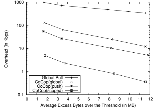
Figure 10: Tradeoff between Average Excess Traffic and Communication Overhead. The curve of CoCop(push) lies about below CoCop(global). CoCop(scoped) is still the lowermost curve.
