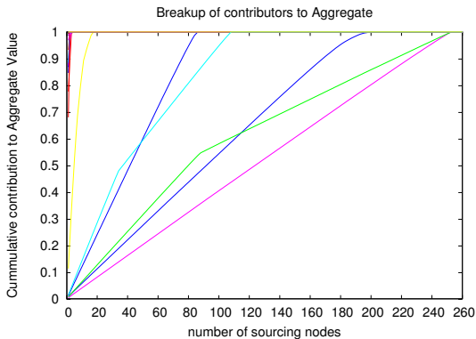
Figure 3: Cumulative composition of anomalous flow aggregates by PlanetLab node. Most anomalies have only one significant contributor and the curves for these overlap as a step function at n=1 . The slanted curves are distributed anomalies.
