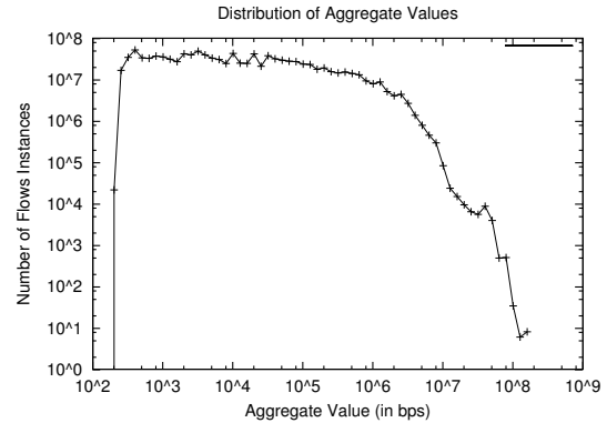
Figure 2: Distribution of Aggregate samples. The distribution is skewed, with very many small samples and very few large samples. Note the log-log scale.
