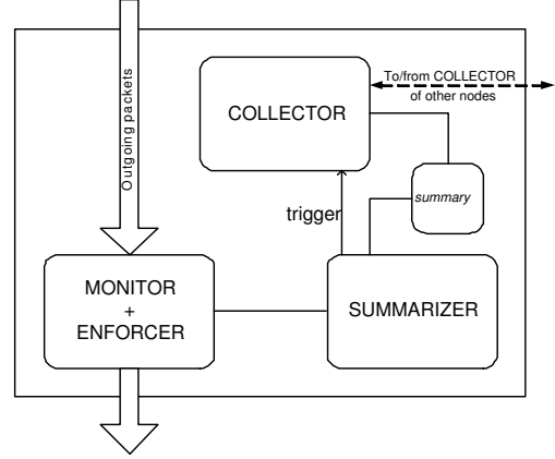
Figure 1: Components of pull-based CoCop at each node
