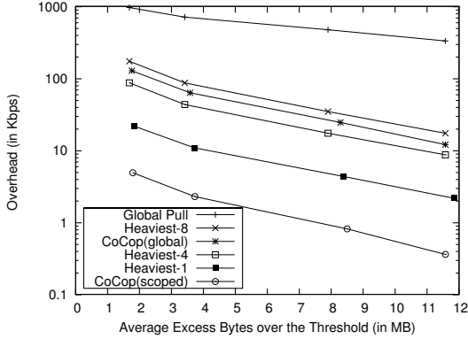
Figure 7: Tradeoff between Average Excess Traffic and Communication overhead for the different mechanisms. The graph illustrates the win-win situation for CoCop(scoped) over the rest.
