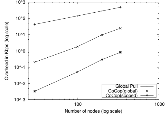
Figure 8: Variation of communication overhead with number of nodes
